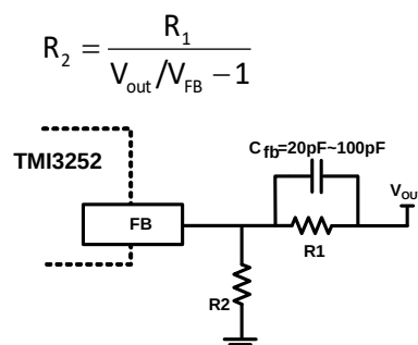
Figure 2. Feedback Network
