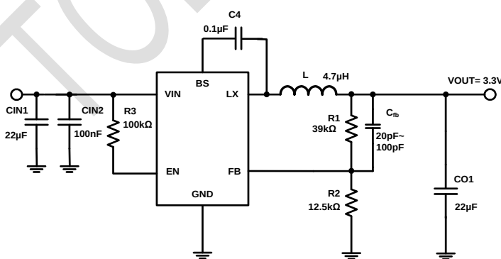
TMI3252 Typical Application Circuits ( V_{REF}=0.8V )
